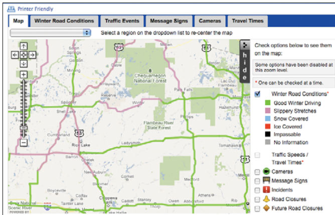
FIGURE 11.1 Full-color vision
